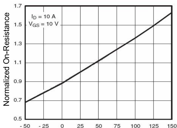
Figure 8 Drain-Source On-Resistance
